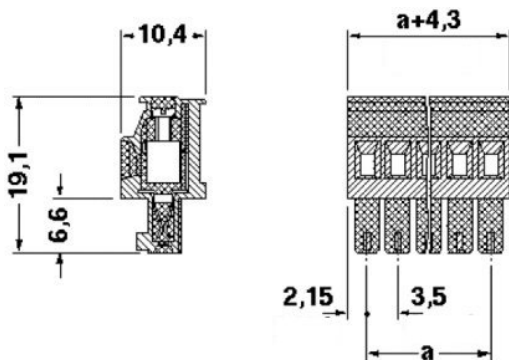
Dimensioned drawing
